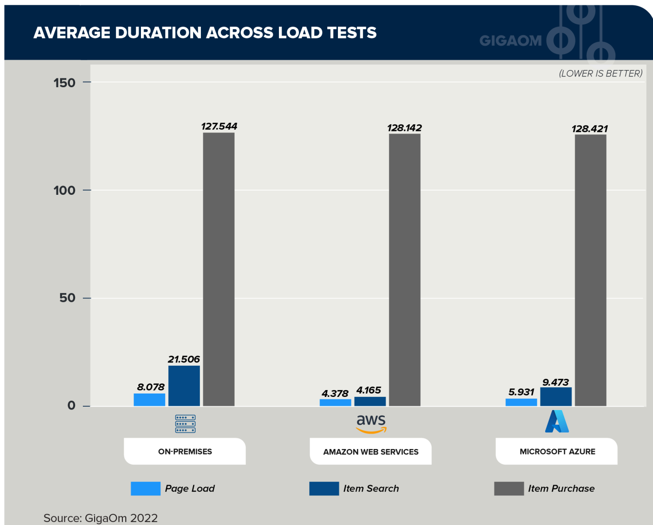
Figure 9. Average Duration Across Load Tests (lower is better)
