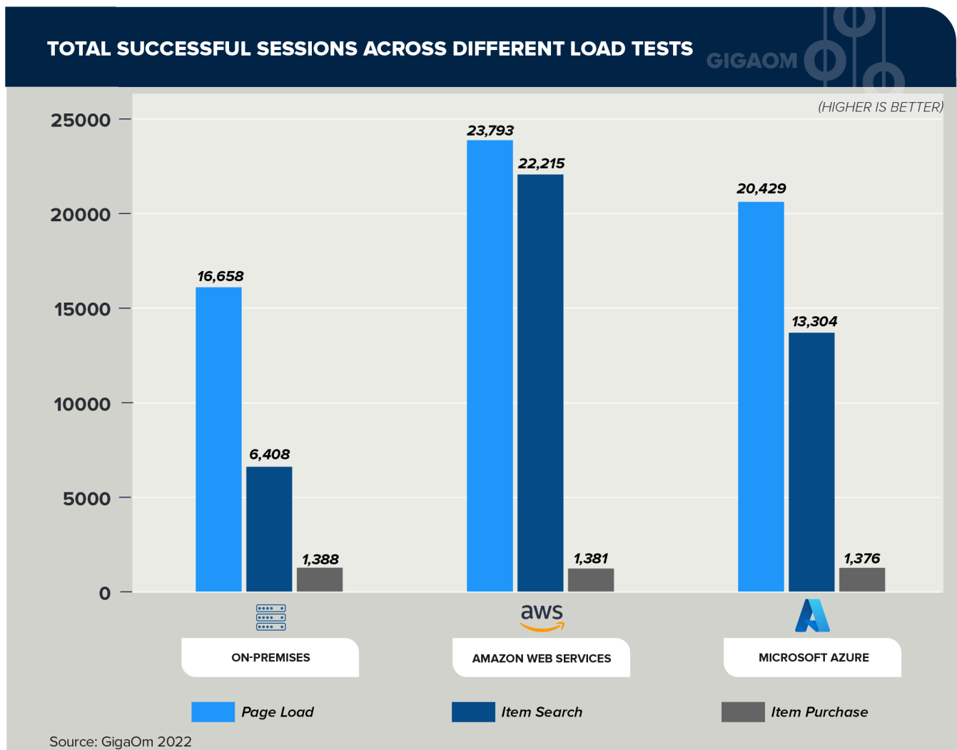
Figure 8. Total Successful Sessions Across Different Load Tests (higher is better)
